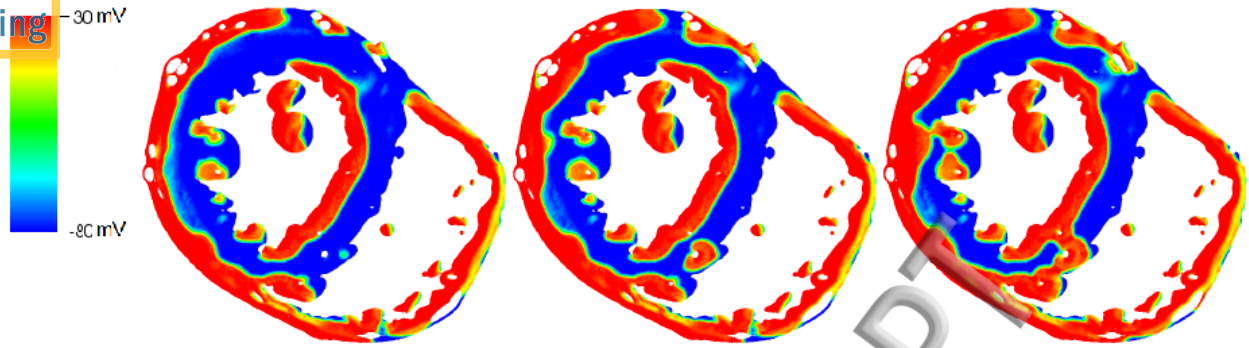
FIG. 8. Transmembrane voltage sensitivity to blood vessel wall conductivity, shown 4 ms after weak shock initiation. Left to right, blood vessel wall conductivities of 0.01, 0.20 and 1.0 S/m. The right frame, with wall conductivity equal to that of blood is equivalent to no wall for the blood vessel.
